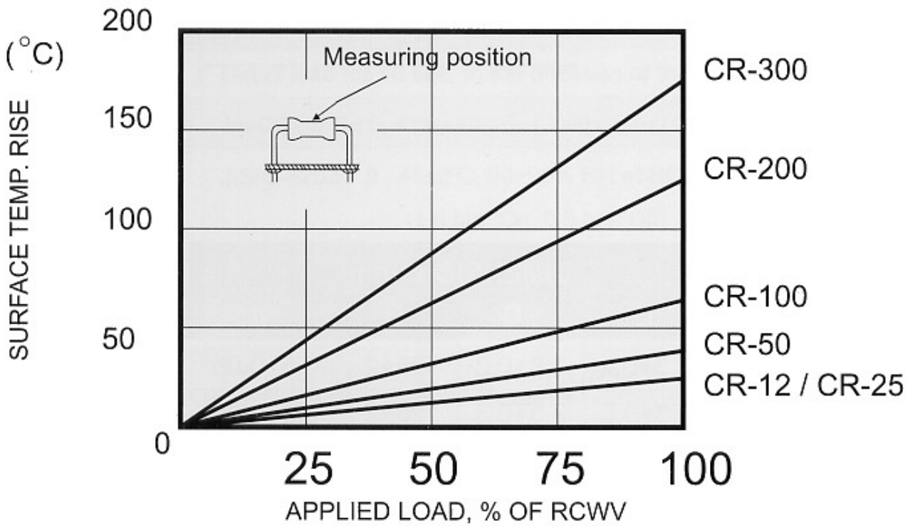
FIG.2 Hot-Spot Temperature
