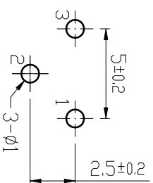
Mounting Hole Details
